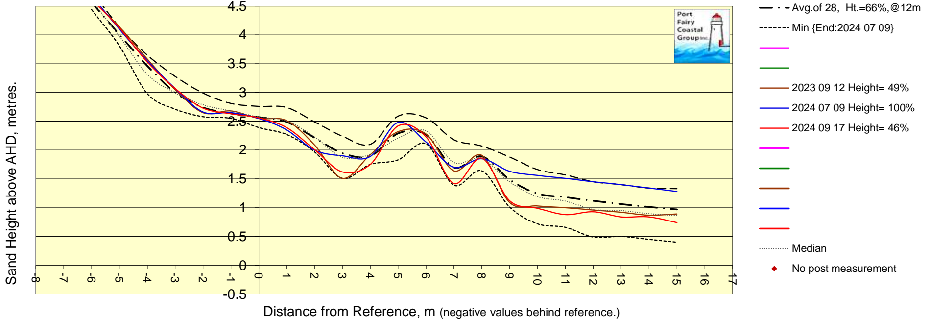
Chart PFETP8.1 Point 8.1 Profile of Dune Toe, WEDs and Foreshore.
