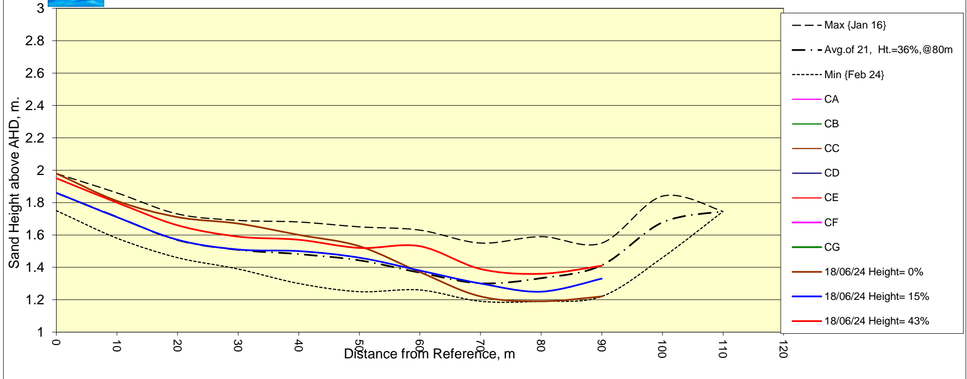
Chart PFSHLP21 Post 21, Longitudinal profile, Pea Soup 3. (Legend date formats: dd/mm/yyyy = laser, yyyy mm dd = Propeller Aero, yymmmdd = GPS)
