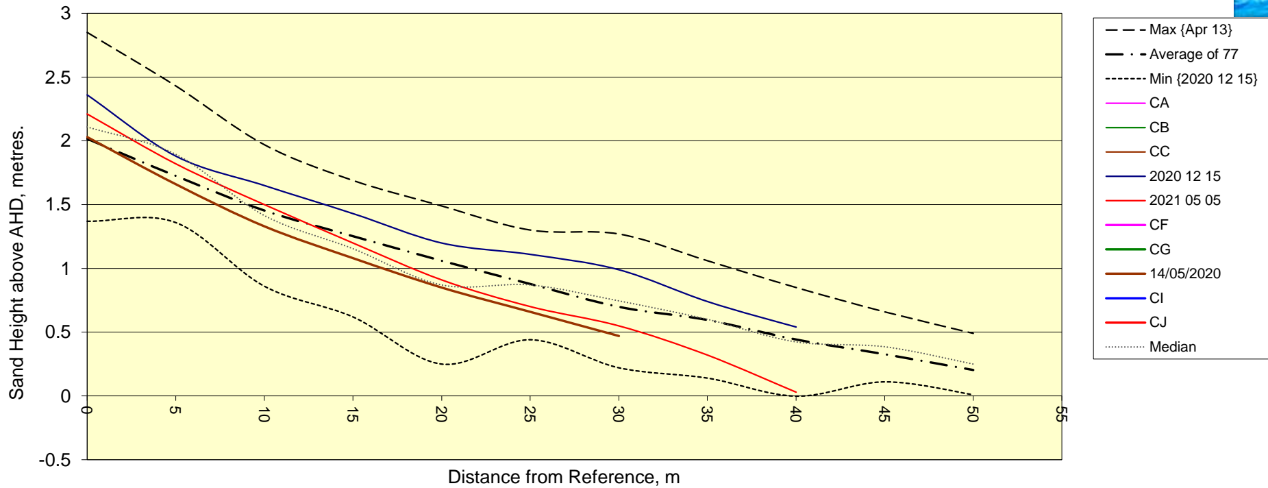
Chart PFEHTP7 Post 7 Transverse Profile perpendicular to dune scarp. (Legend date formats: dd/mm/yyyy = laser, yyyy mm dd = Propeller Aero, dd mmmmyy = GPS) {Stats date range in braces}
