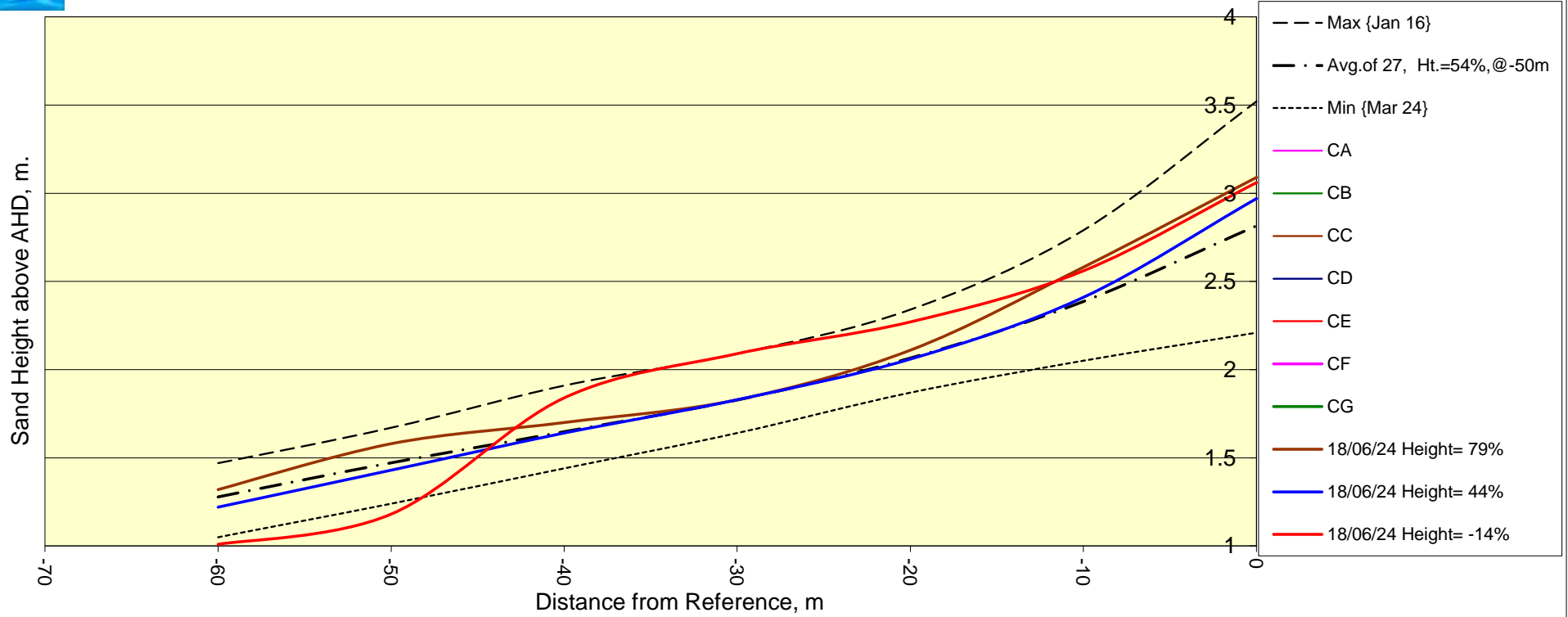
Chart PFSHLP23 Longitudinal Profile oblique to Dog Beach (Legend date formats: dd/mm/yyyy = laser, yyyy mm dd = Propeller Aero, yymmmdd = GPS)
