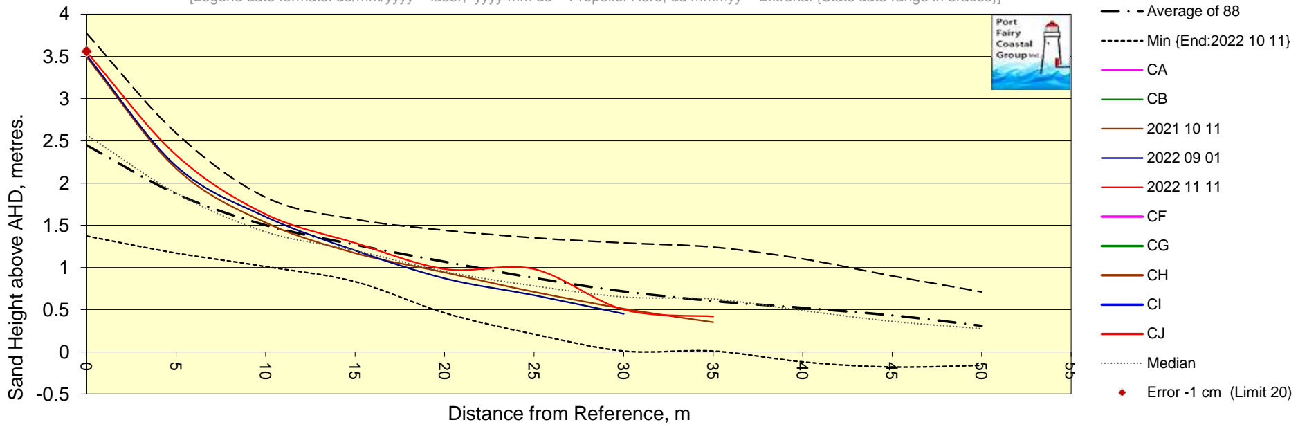
Chart PFETP5 Post 5 Transverse Profile perpendicular to dune scarp.
