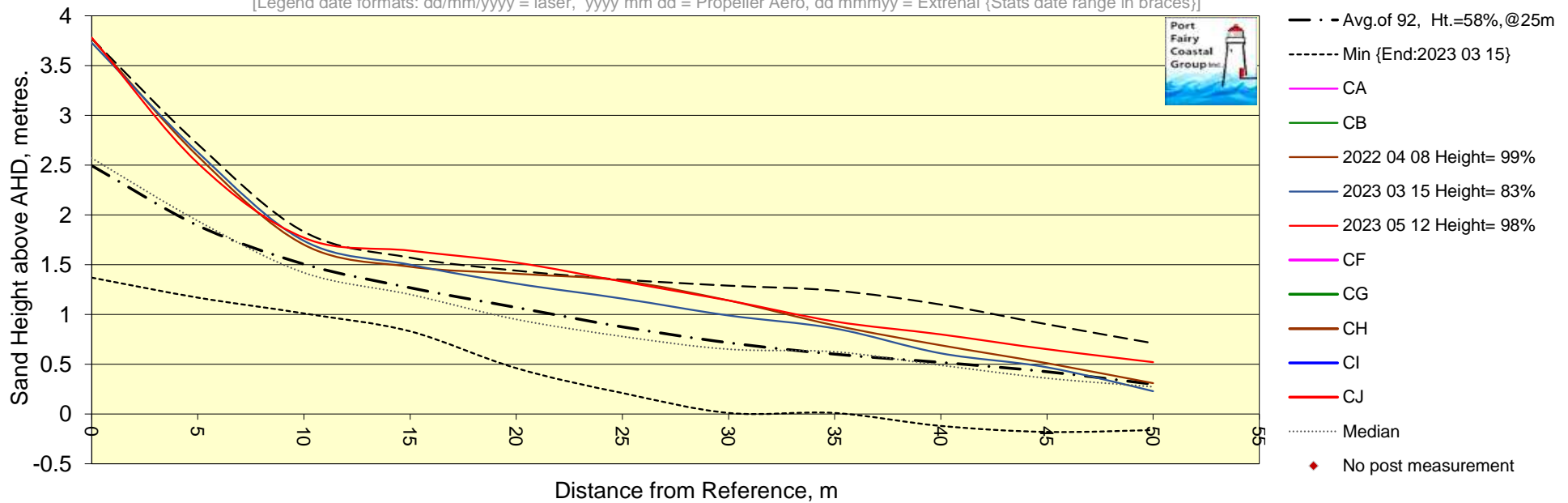
Chart PFETP5 Post 5 Transverse Profile perpendicular to dune scarp.
